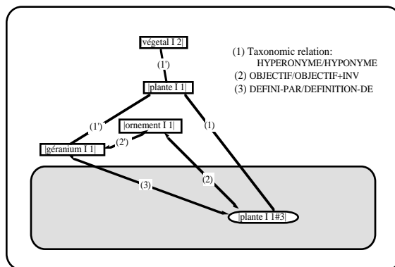
Fig. 2. Relational view of the concept |géranium I 1| (in the THESAURUS net).
