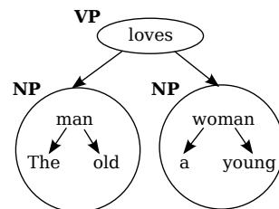
Figure 2: An example of the dependency tree structure: “The old man loves a young woman”.
